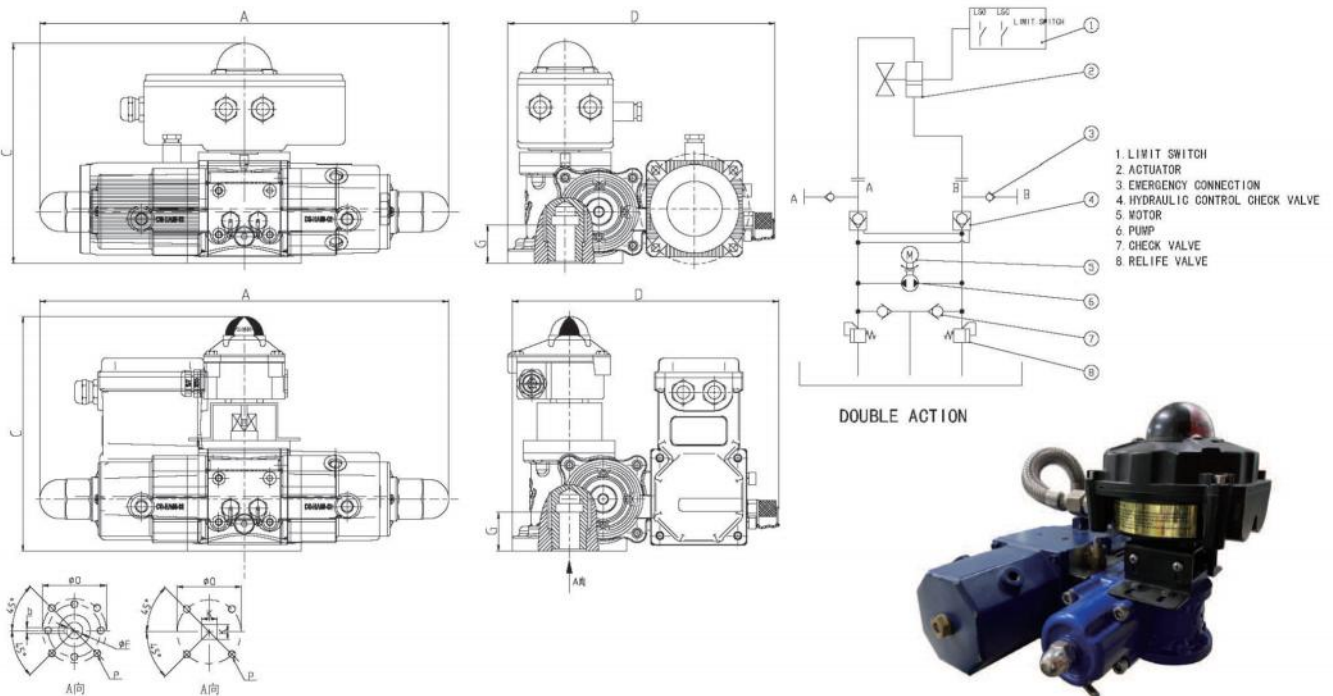
外形及连接尺寸 SHAPE AND CONNECTING DIMENSIONS (mm)
