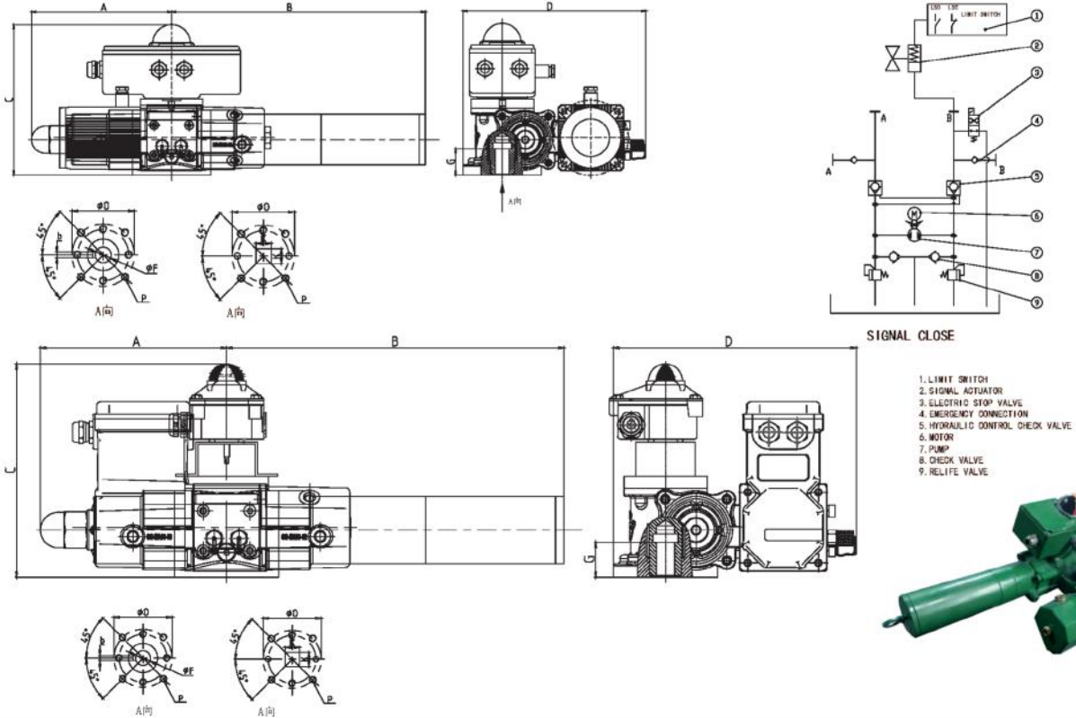
外形及连接尺寸 SHAPE AND CONNECTING DIMENSIONS (mm)
